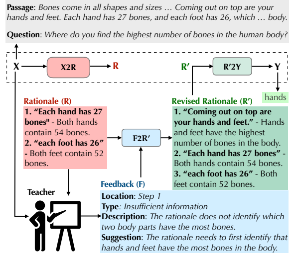
Figure 1: The framework for incorporating human feedback into decomposed QA models. A model X2R generates a rationale R to answer a question based on a passage. A human teacher then provides natural language feedback for R , which is used to generate a revised rationale R' from F2R' . Finally, this revised rationale is used to generate the final answer Y . We study various formats of the intermediate rationale R .
